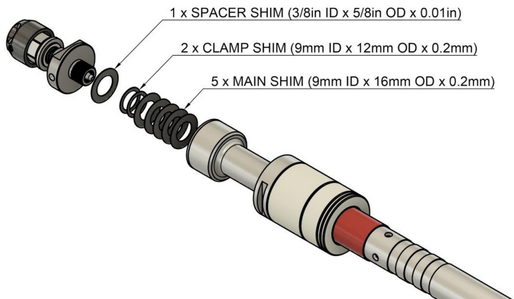
DRAWING 3: Stock shim stack configuration
