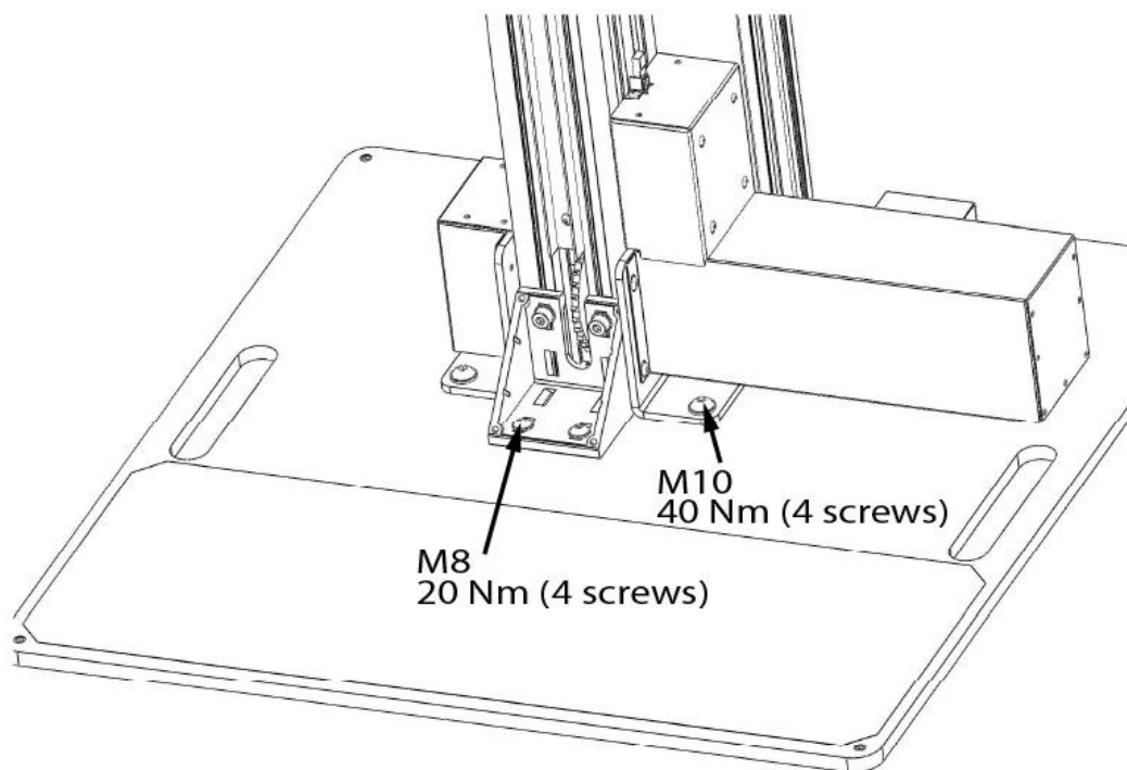
Figure 3: Stand mounting screws
