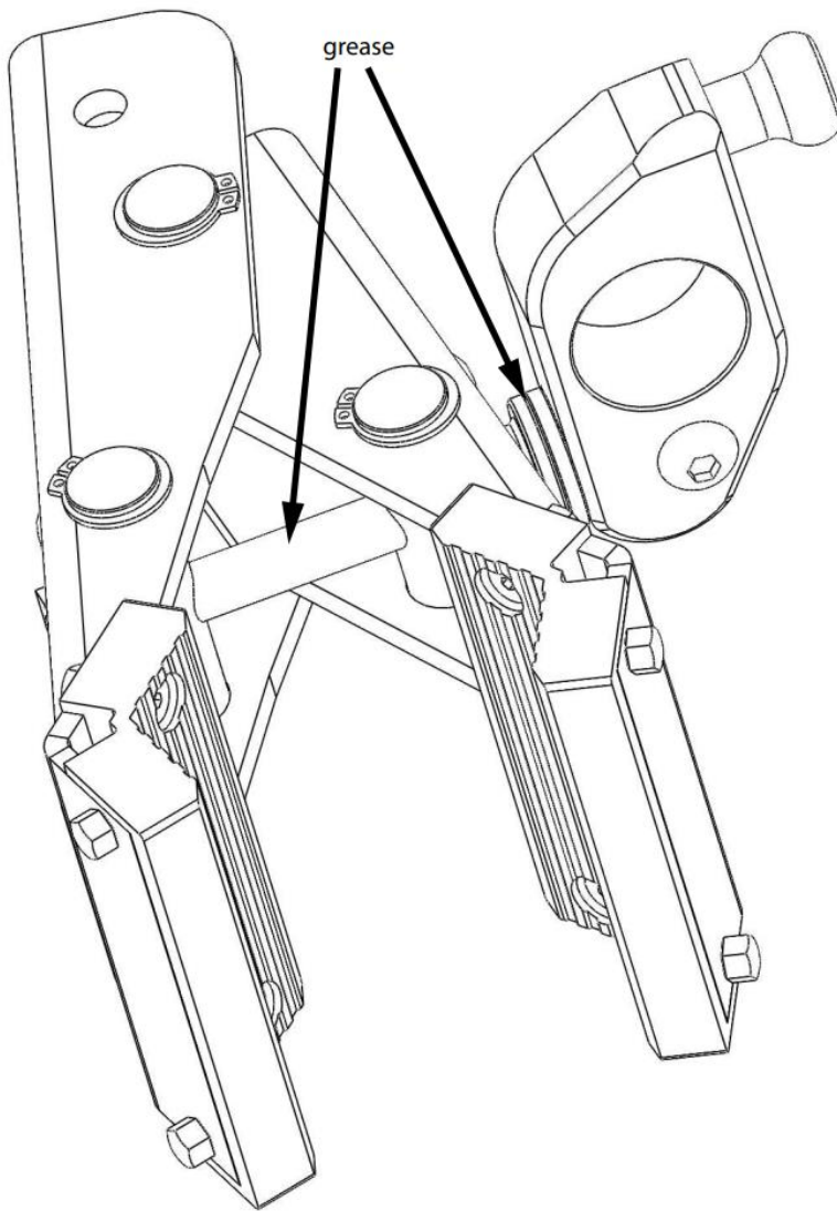
Figure 10: Clamp grease location
