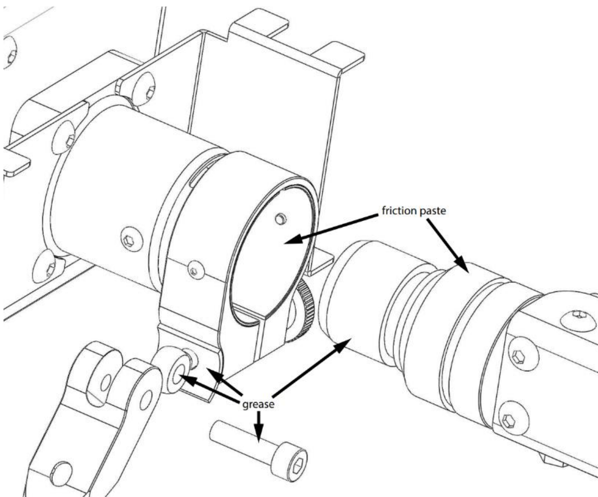
Figure 9: Clamp Holder grease and friction paste locations
